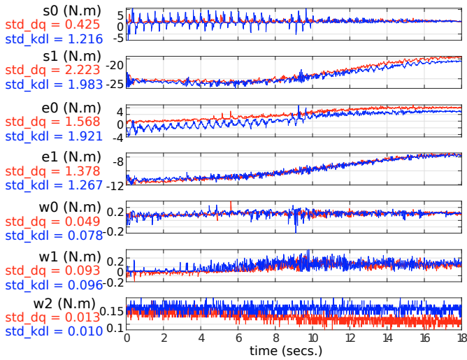
Fig. 5. Joint Effort plot for the coupled (—) and decoupled (—) controllers. std_dq and std_kdl refers to the standard deviation of the joint efforts for coupled approach and decoupled approach, respectively.
